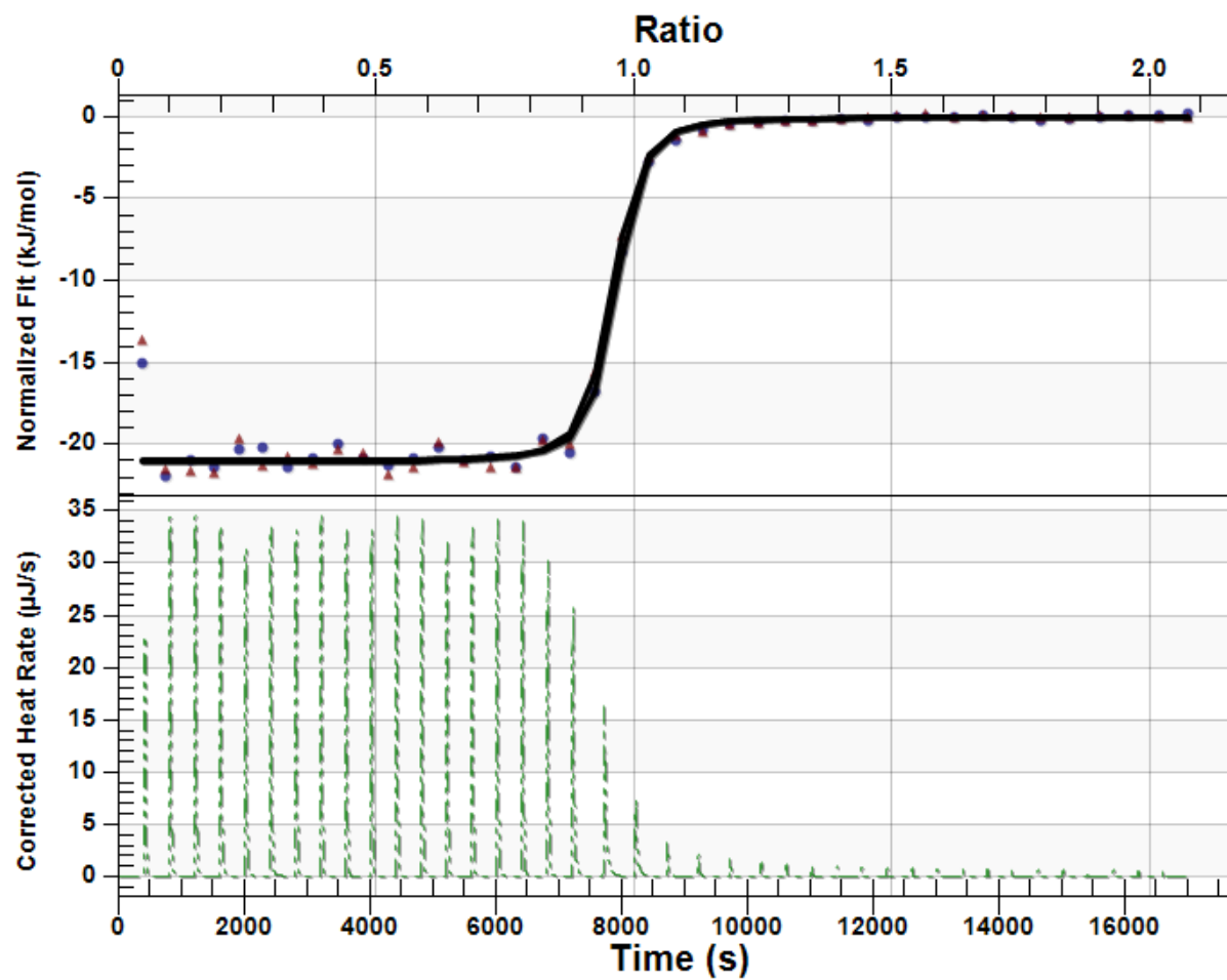
Figure C-18: ITC Thermogram of 4 z ,5' z cis-syn-cis -di- tert -butylcyclohexano-18-crown-6 Complexed with \text{SrCl}_2 \cdot 6\text{H}_2\text{O} in Anhydrous Methanol
