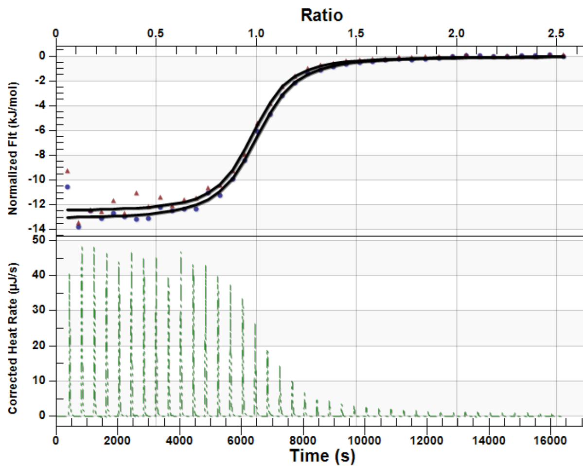
Figure C-9: ITC Thermogram of DCH18C6D Isomer Complexed with \text{SrCl}_2 \cdot 6\text{H}_2\text{O} in Anhydrous Methanol
