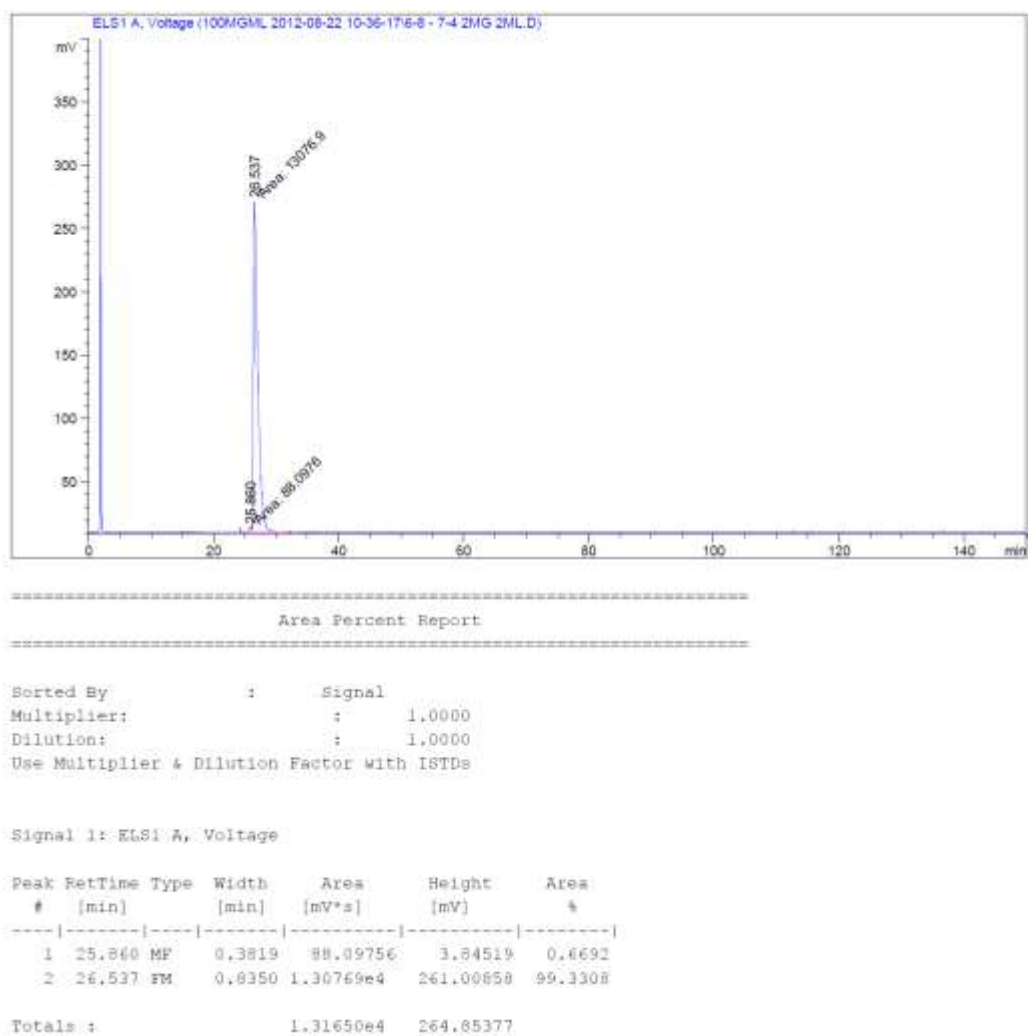
Figure D-23: Chromatogram of Prep Sample Fraction 6.8-7.4 Minutes
