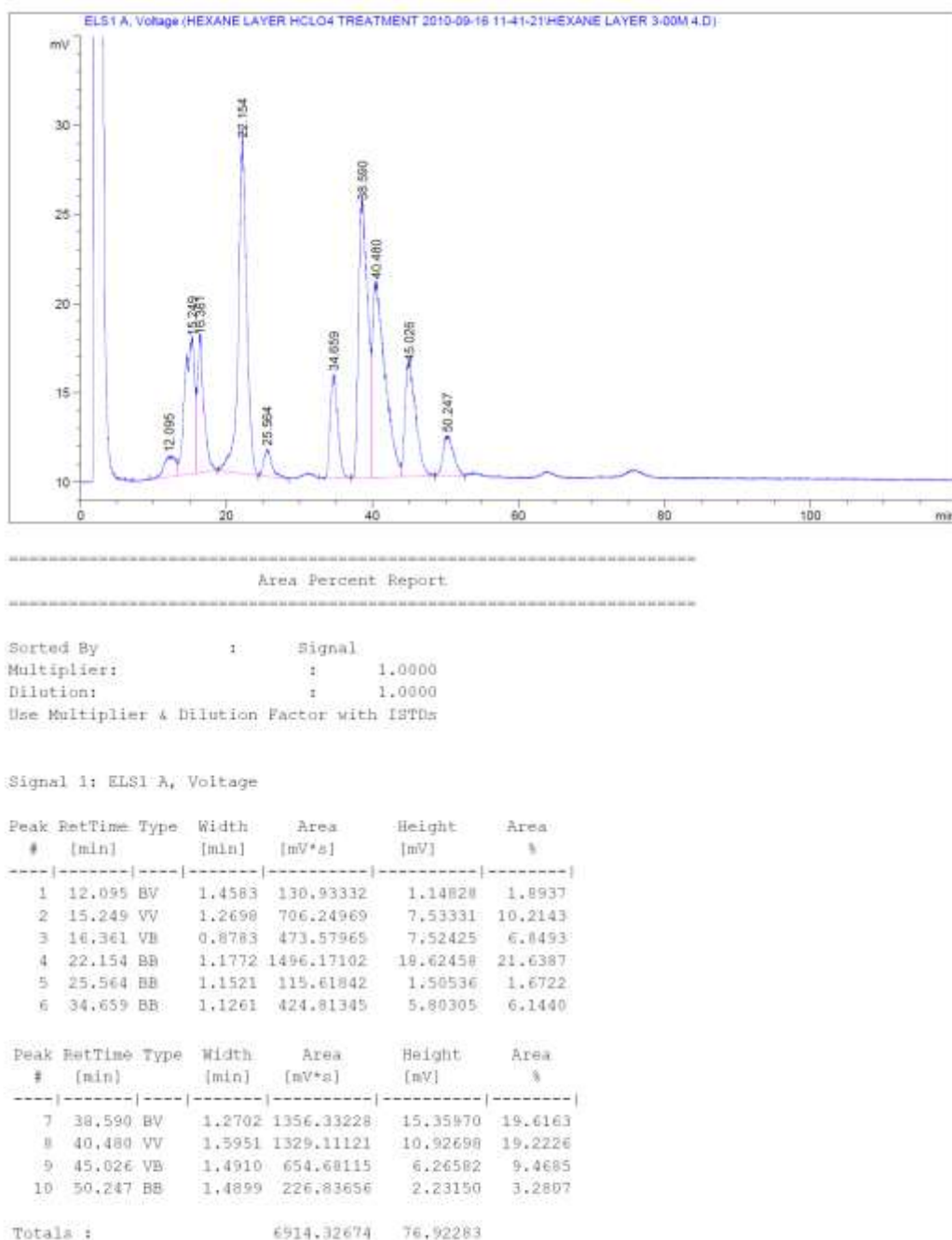
Figure D-10: 3.00M Hexane Layer Containing Uncomplexed Crown Ether and Contaminants
