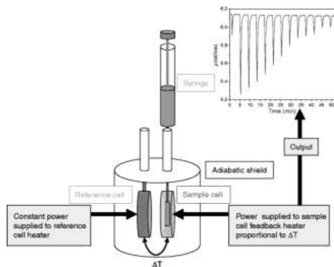
Figure 4.2: Schematic of Isothermal Titration Calorimetry (14)
