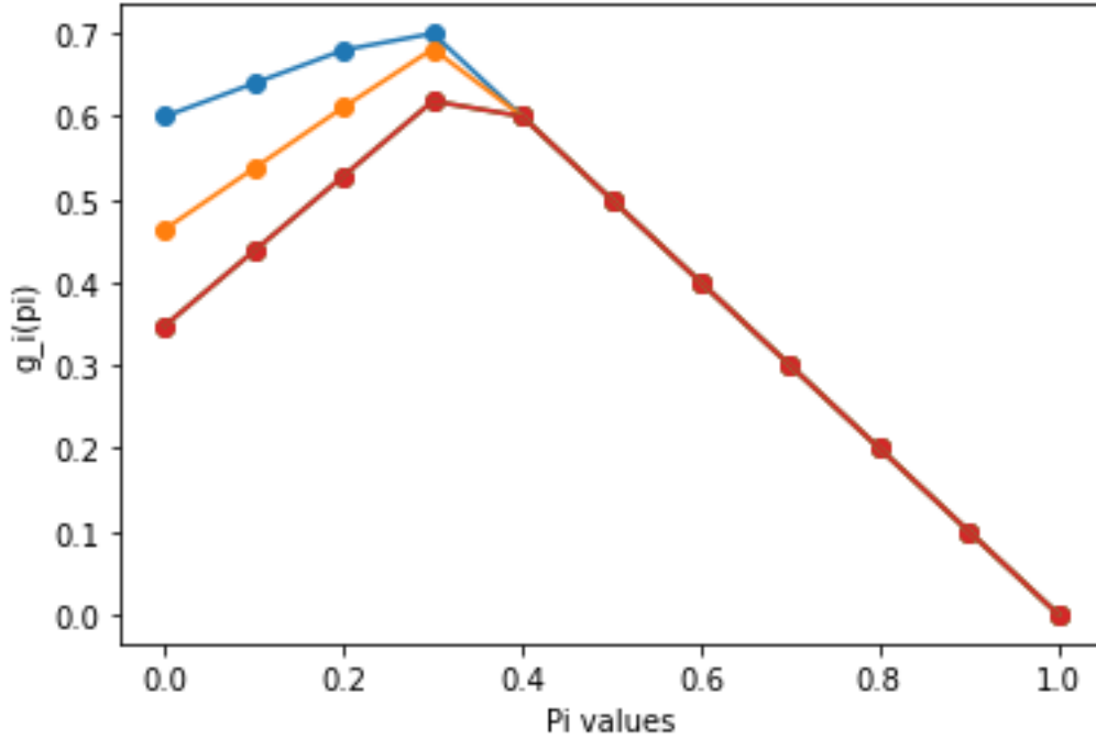
Figure 5.2: Interpolation between the calculated values of Qg(\pi) with blue: Q(\pi) , orange: Q^2 and red: Q^{1000} .
