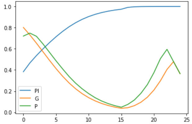
Figure 6.4: Simulation 2: \pi , g(\pi_{n,B}, \pi_{n,C}) and \rho
