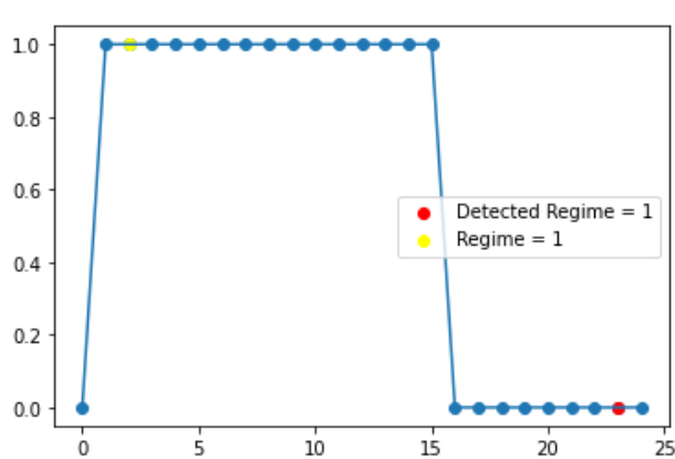
Figure 6.3: Simulation 2: Markov chain values
