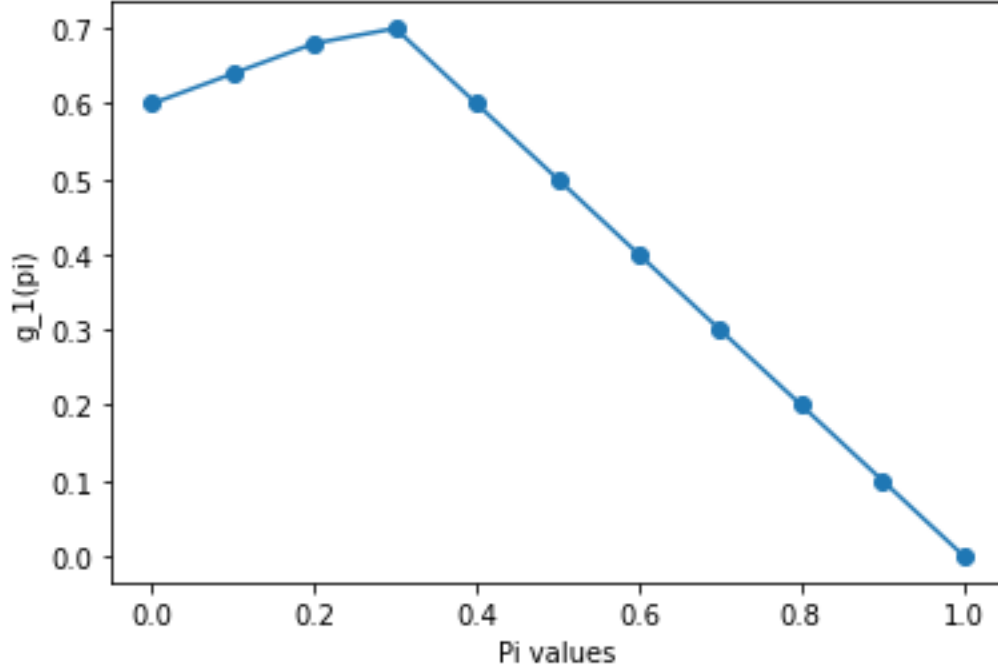
Figure 5.1: Interpolation between the calculated values of Qg(\pi)
