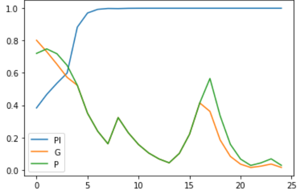
Figure 6.2: Simulation 1: \pi , g(\pi_{n,B}, \pi_{n,C}) and \rho
