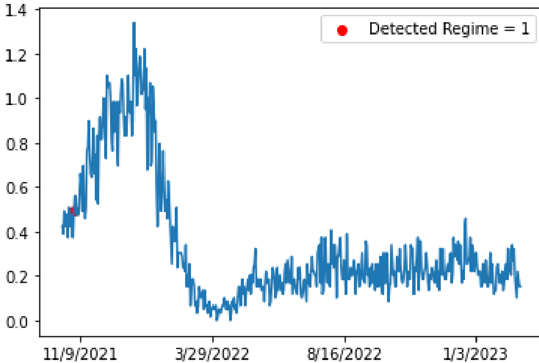
Figure 7.8: Change Point Detection on Wisconsin Hospital Data (Age 60-69) with start date on October 31st 2021
