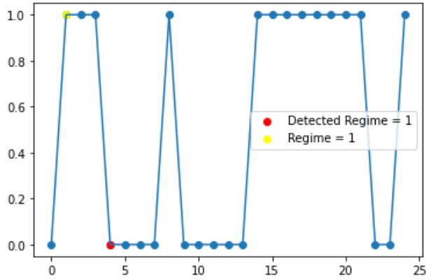
Figure 6.1: Simulation 1: Markov chain values
