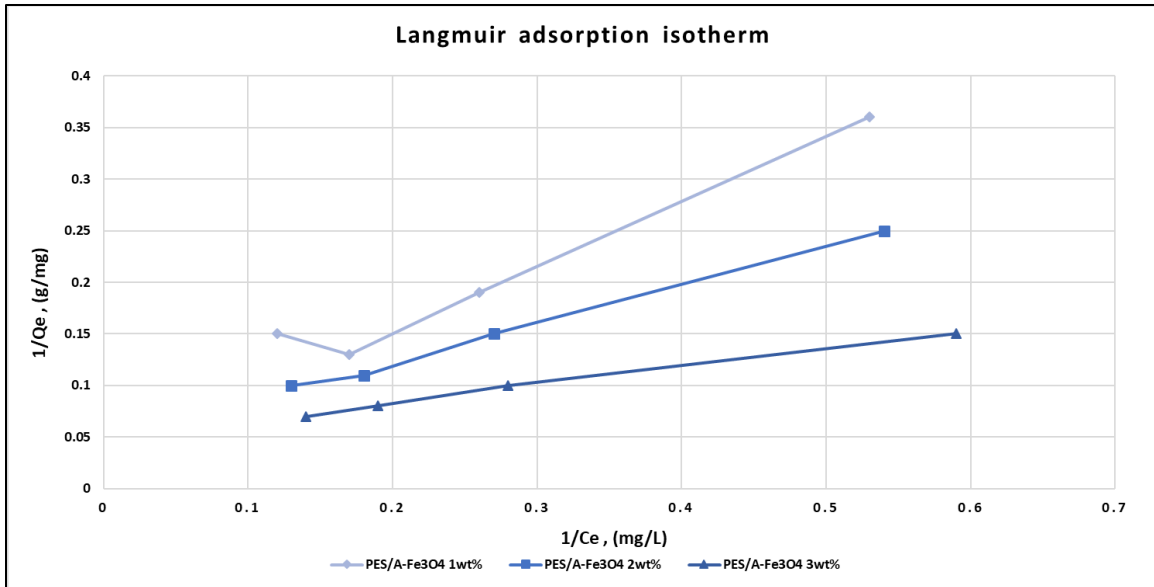
Figure 3.14 Langmuir adsorption isotherm of nanocomposite membranes, conditions: T=25 °C, pH=2
