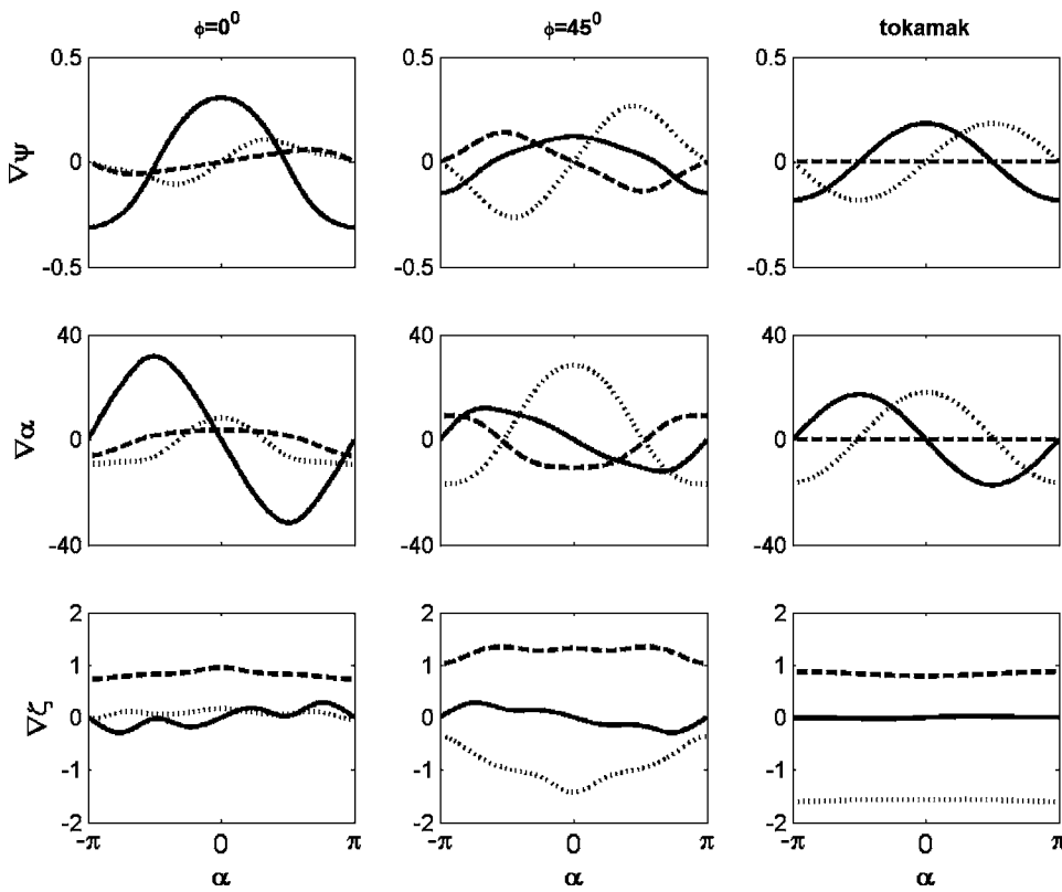
FIG. 1. The components of the contra-variant basis set in HSX for a flux surface with r/a \sim 0.5 at toroidal locations \phi=0^\circ and \phi=45^\circ , as well as for the equivalent tokamak based on the large-aspect-ratio approximation given in Ref. 7. The curves correspond to the component of the vector in the \hat{R} ( P , solid line), \hat{Z} ( G , dotted line), and \hat{\phi} ( Q/R , dashed line) directions, and are plotted as a function of the Hamada poloidal angle \alpha .
