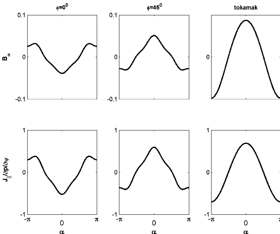
FIG. 6. Numerical calculation of B_\alpha and J_\parallel/dp/d\psi = (2\pi B_\alpha/B) for HSX at \phi=0^\circ and \phi=45^\circ compared to the analytic tokamak approximation.
