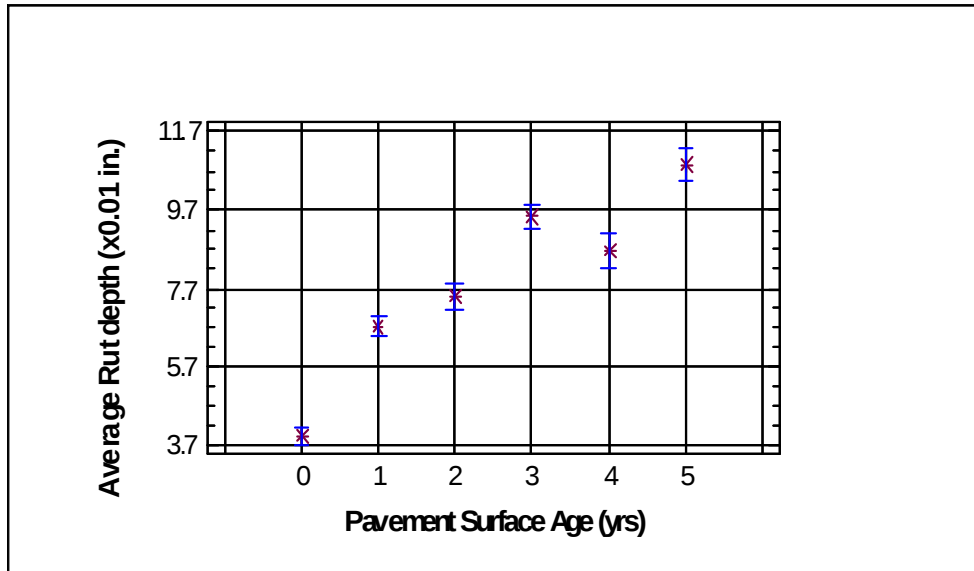
Figure 5.1 Means and 95% LSD Intervals for Rut Depth Progression by Age
