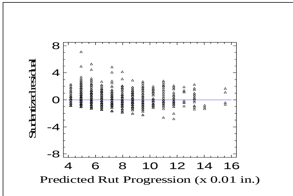
Figure 5.3 Studentized Residual Plot Prior to Accounting for Outliers.
