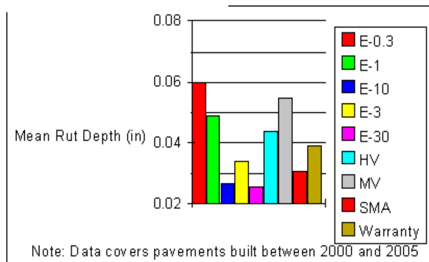
Figure 4.6 Average Rut Depths for Newly Constructed Pavements
