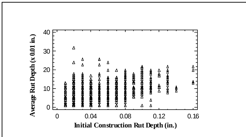
Figure 5.2 Basic Scatter Plot of Rut Progression after Initial Construction
