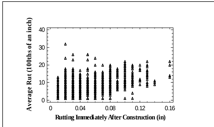
Figure 4.10 Rutting Progression Based on Initial Rut Depth at Construction
