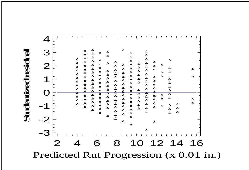
Figure 5.4 Studentized Residual Plot After Accounting for Outliers.
