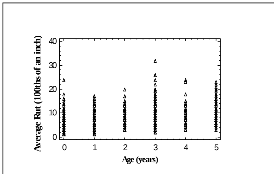
Figure 4.9 Mean Rut Depth Variations with Surface Age
