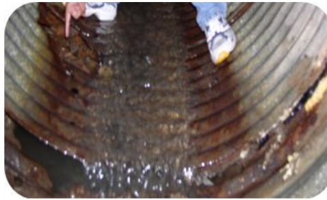
Figure 9.1: Big Hole and Corrosion in the Invert of the Culvert 25001273A01
