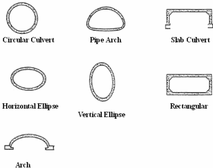
Figure A2.2: Different Shapes of Culverts If the culvert is circular, code “01”
