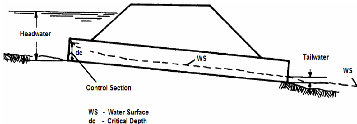
Figure 2.6: Typical Flow in a Partially Full Culvert (Source: FHWA, 2001)
