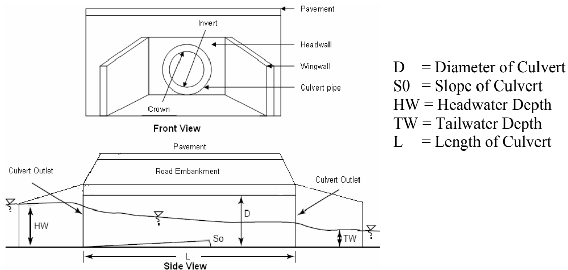
Figure 8.2: Components of a Culvert
