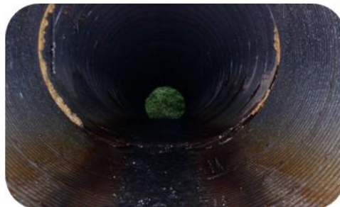
Figure 9.2: Misalignment of the Culvert 25001273A01
