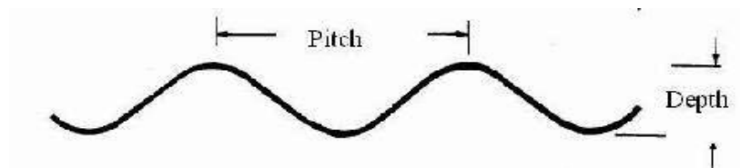
Figure A1.3: Pitch of Corrugated Metal Culverts
