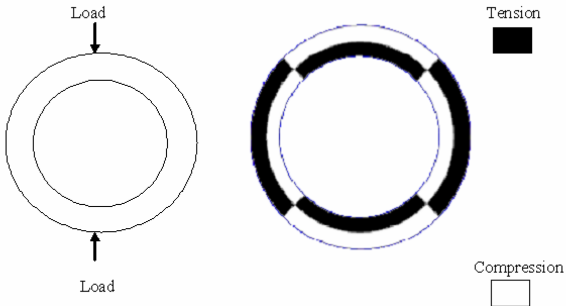
Figure 2.8: Zones of Tension and Compression in Rigid Pipes
