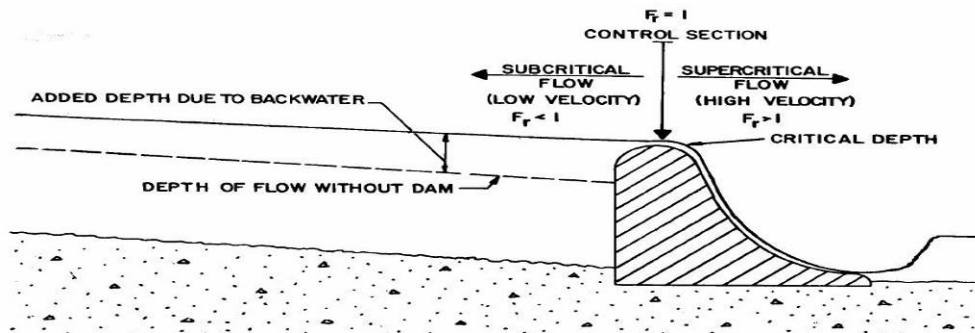
Figure 2.5: Flow Conditions for a Small Dam (Source: FHWA, 2001)
