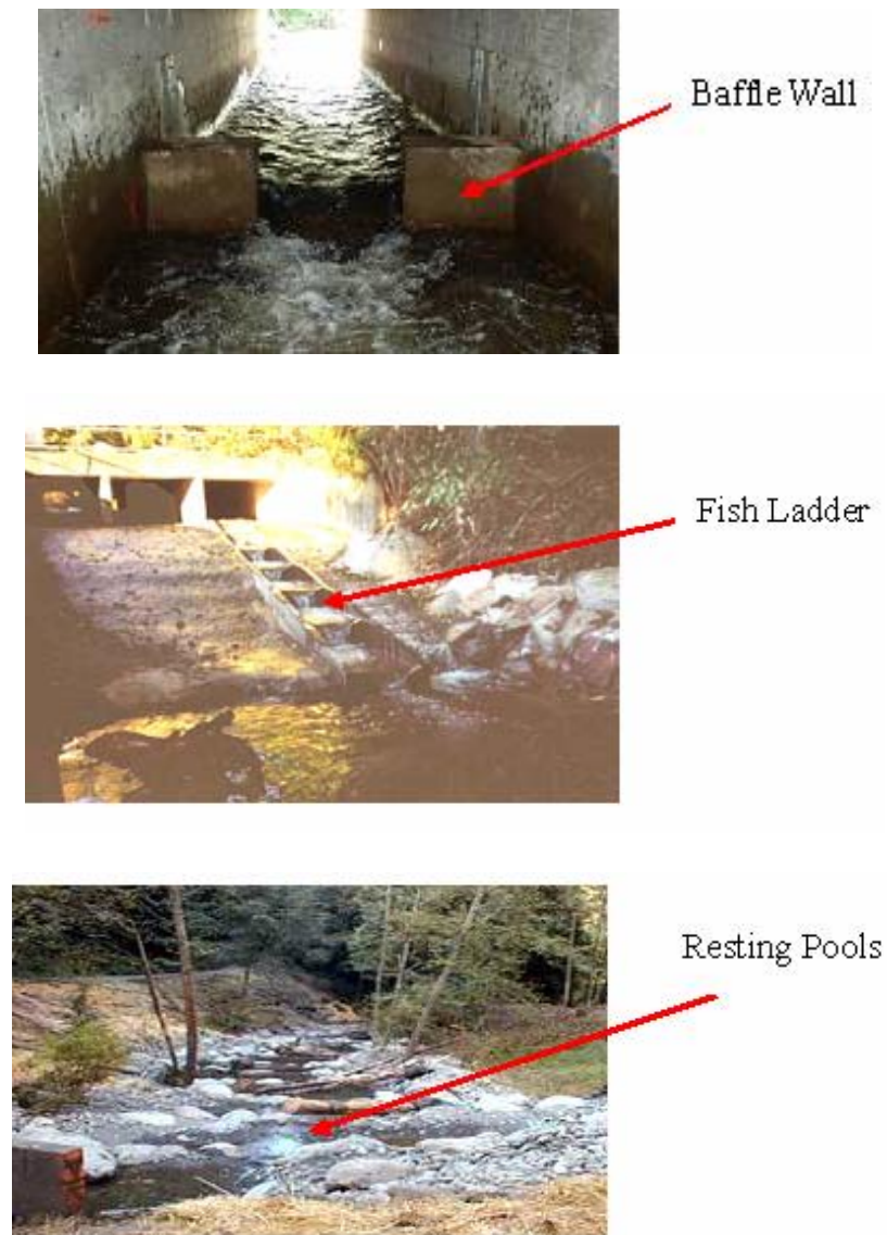
Figure A2.7: Types of Fish Ladders
