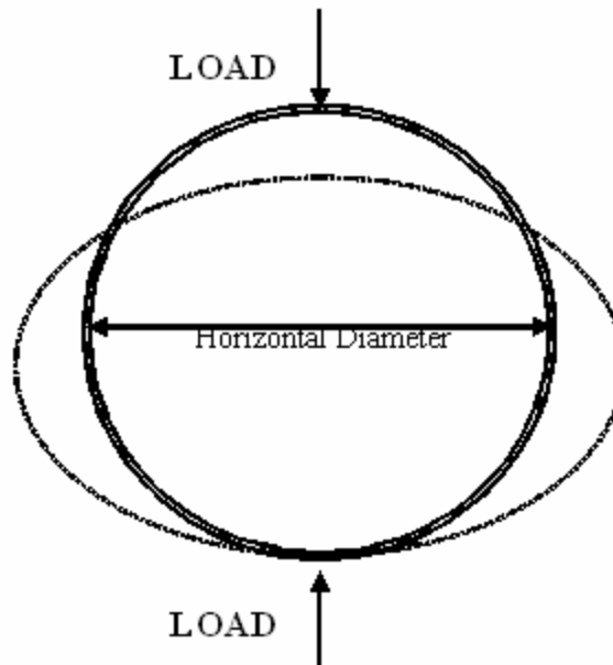
Figure 2.7: Deflection of Flexible Culverts (Source: FHWA, 1986)
