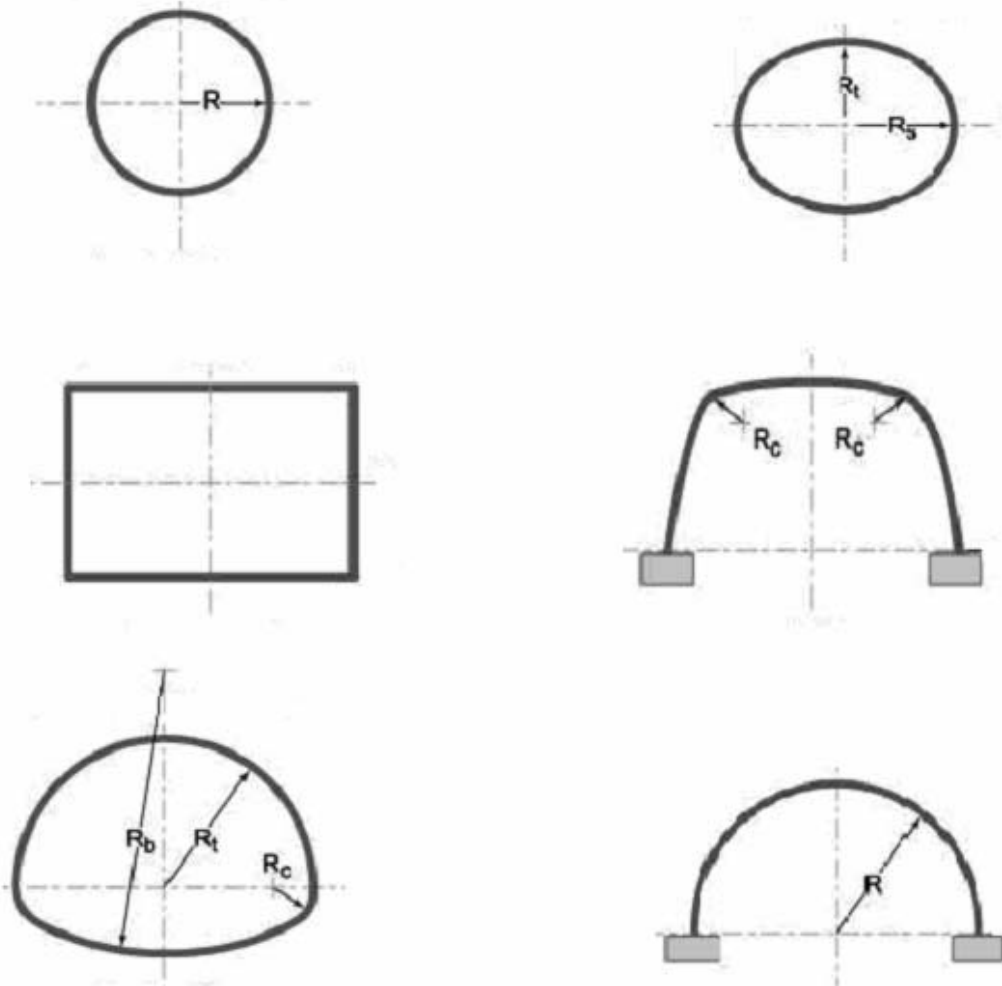
Figure A1.2: Geometric Dimensions of Culverts
