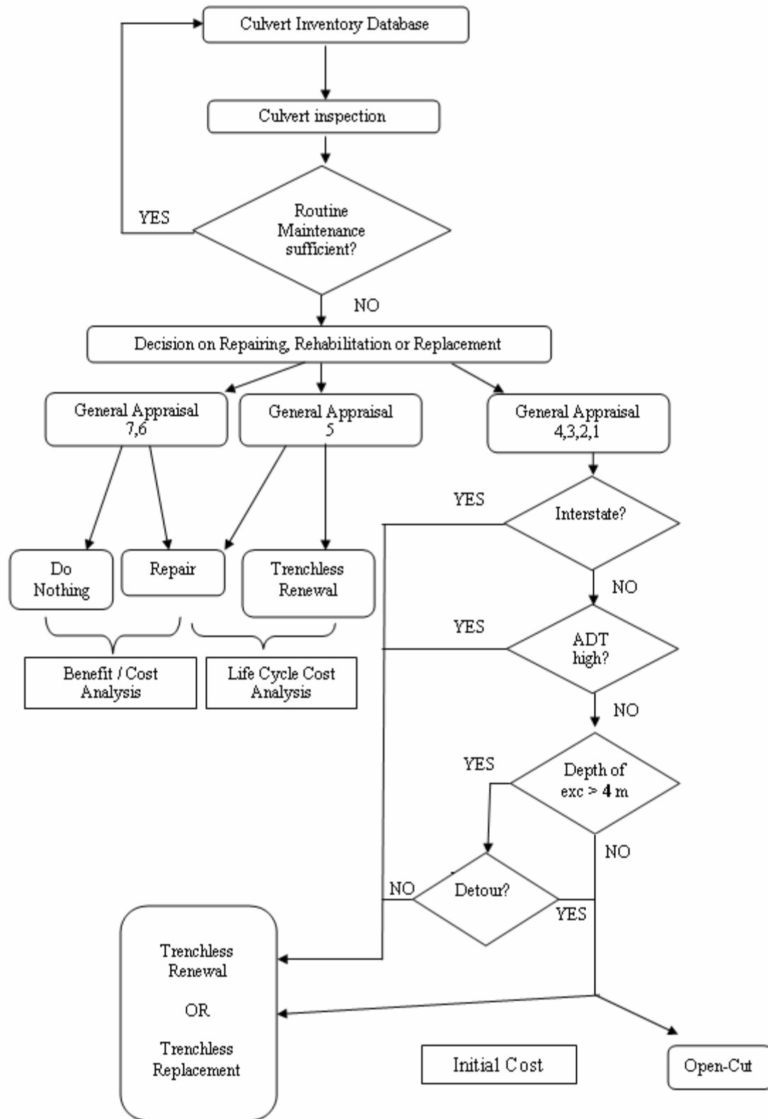
Figure 6.1: Culvert Asset Management Decision Platform.
