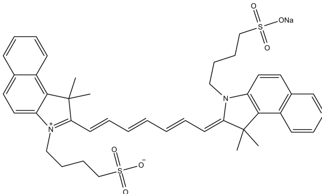
sodium 4-[2-[(1E,3E,5E,7Z)-7-[1,1-dimethyl-3-(4-sulfonatobutyl)benzo[e]indol-2-ylidene]hepta-1,3,5-trienyl]-1,1-dimethylbenzo[e]indol-3-ium-3-yl]butane-1-sulfonate (Indocyanine green)
