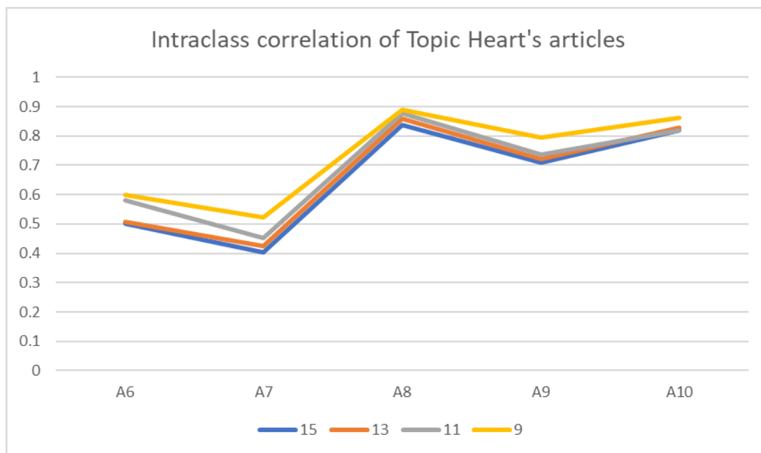
Figure 20. The intraclass correlation coefficients of Topic Heart's articles for different list sizes
