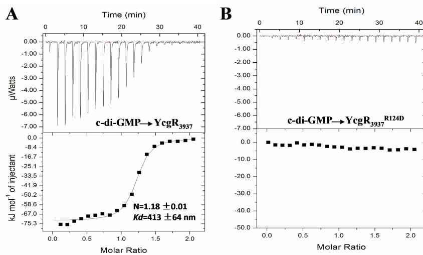
FIG 5 Isothermal titration calorimetric analysis of c-di-GMP binding to wild-type YcgR 3937 (A) or the point mutation version YcgR 3937 R124D (B). Calorimetric titration for c-di-GMP (500 μM) titrated into test proteins (50 μM) is shown. Derived values for K_d and stoichiometry ( N ) are shown.
