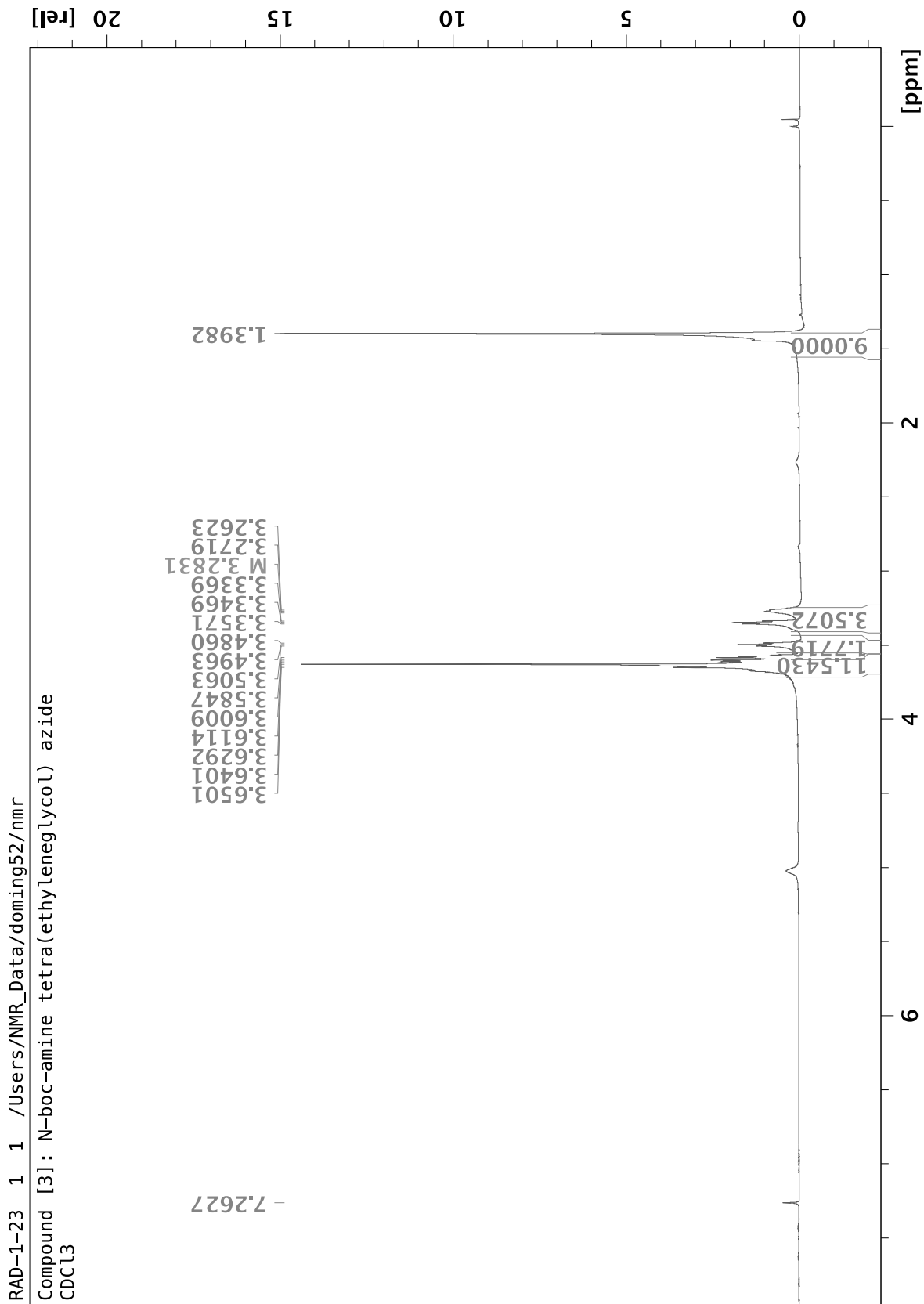
Spectrum 1:Compound [3] 1 H NMR (500 MHz CDCl 3 )
