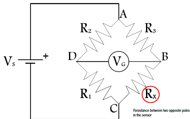
Figure 4. Wheatstone bridge.
