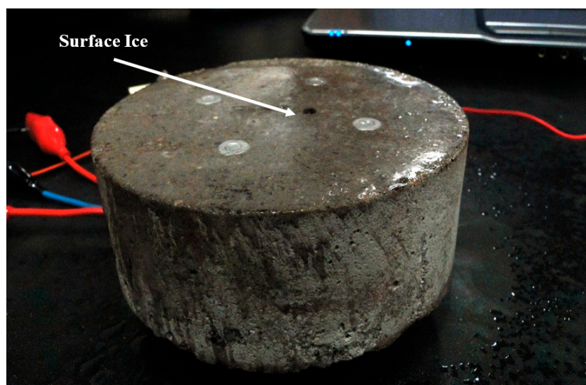
Figure 8. Surface ice formation on cold SP-I sensor.
