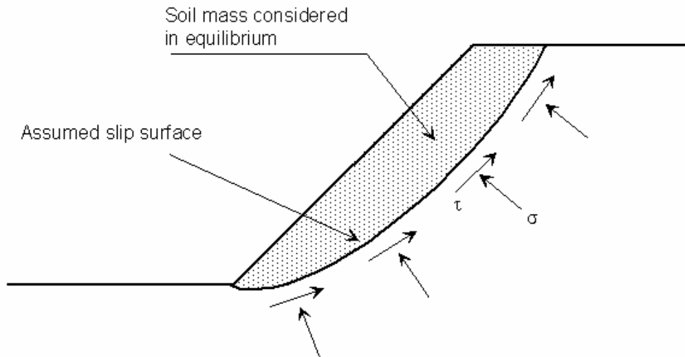
Figure 3.1: Slope with assumed slip surface used for equilibrium analysis in slope stability.
