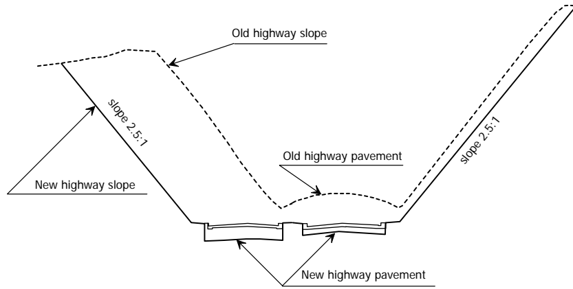
(a) Cross-section of the reconstructed highway at Sta. 299+00
