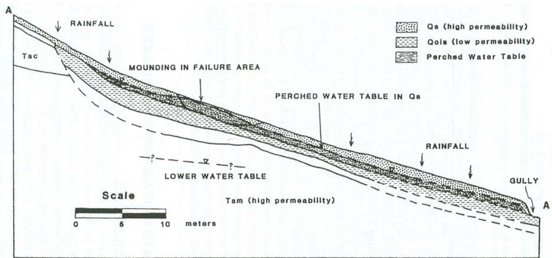
Figure 2.8: Schematic of localized mounding in the failure area with a transient, perched water table in the soil overlying the lower permeability old landslide deposit (Reid et al., 1988).
