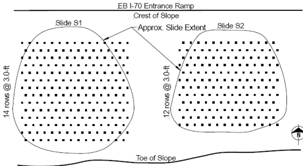
Figure 3.21: Plan view of slide areas S1 and S2 at the I-70 Emma site showing a selected layout of reinforcing members (Loehr and Bowders, 2007).
