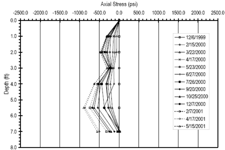
Figure 3.24: Measured incremental axial stress in instrumented member IMG in slide area S1 at I-70 Emma site during Phase I (Loehr and Bowders, 2007).
