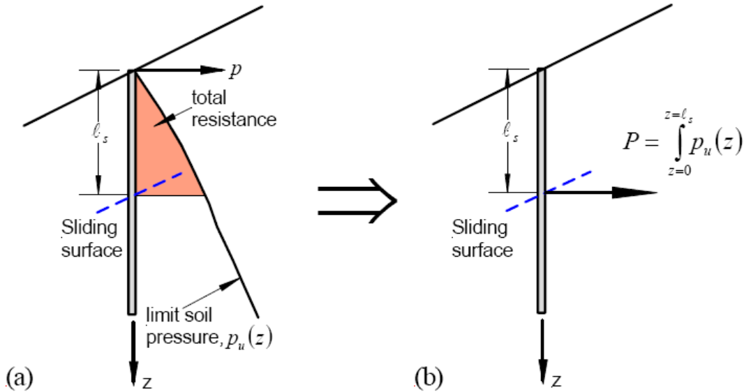
Figure 3.7: Schematic illustrating calculation of limit resistance force: (a) limit soil pressure and (b) equivalent lateral resistance force (after Loehr et al. 2007).
