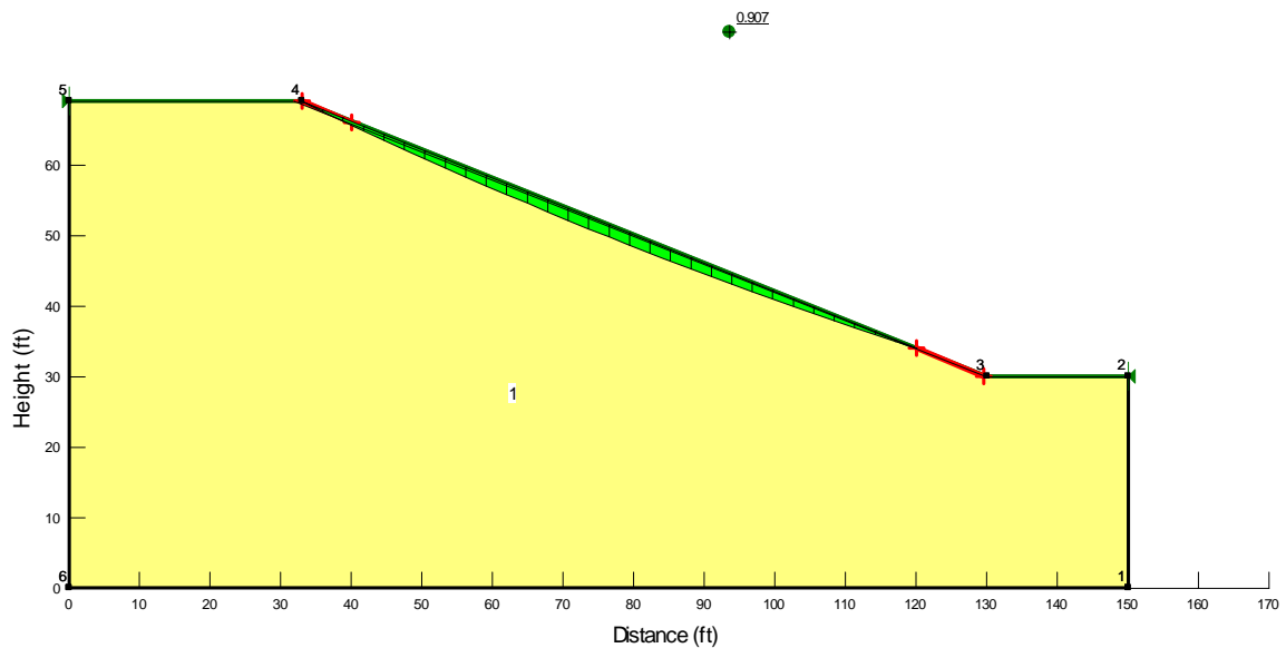
Figure 3.31: Surficial slip surface of the STH-164 slope with dry homogeneous cohesionless soil ( \phi'=20^\circ ).
