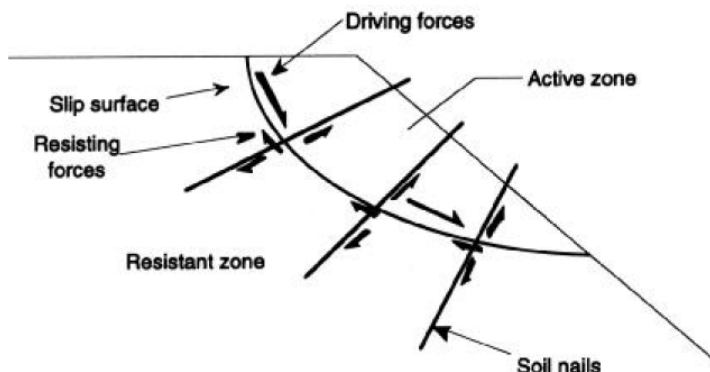
Figure 2.20: Application for soil nails in slope stabilization (FHWA, 2003).
