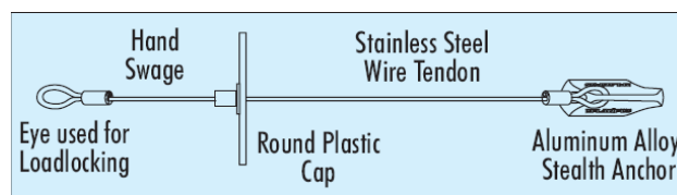
(a) S02E anchor with maximum capacity of 550 lbs.
