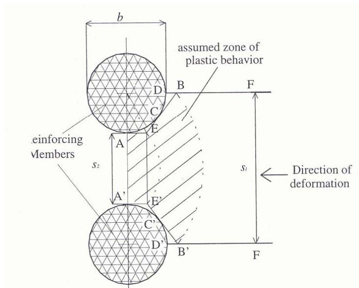
Figure 3.12: Assumed zone of plastic behavior between adjacent piles in a row (after Ito and Matsui, 1975).
