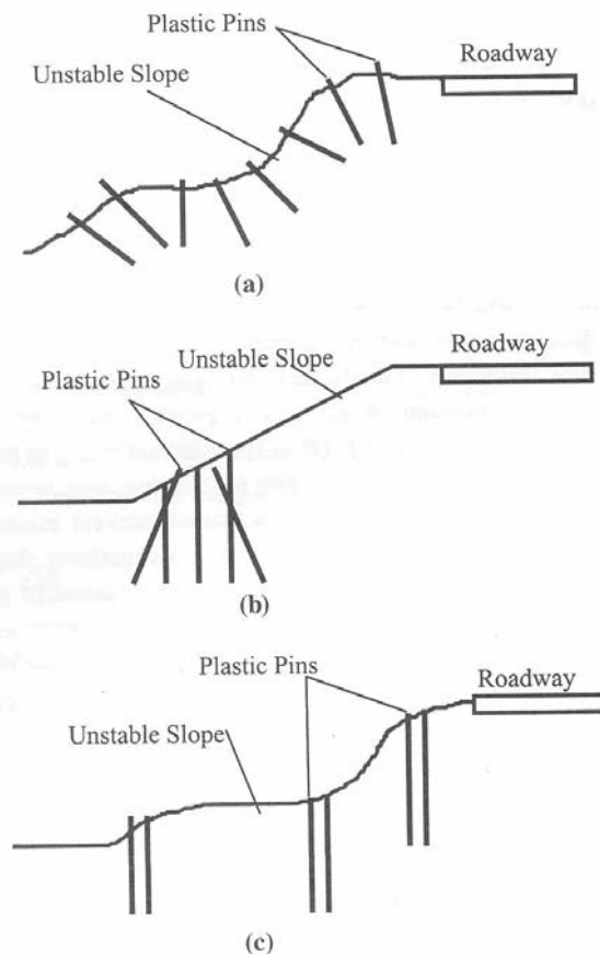
Figure 2.13: Potential schemes for slope stabilization using structural members: (a) soil nailing, (b) reticulated buttress, and (c) soil doweling (after Loehr et al., 2000).
