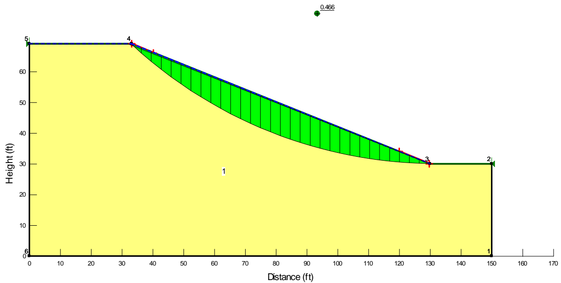
Figure 3.34: Relatively deep slip surface of the STH-164 slope obtained when analysis is conducted with saturated soft homogeneous soil layer ( c' = 20 psf and \phi' = 20^\circ ).
