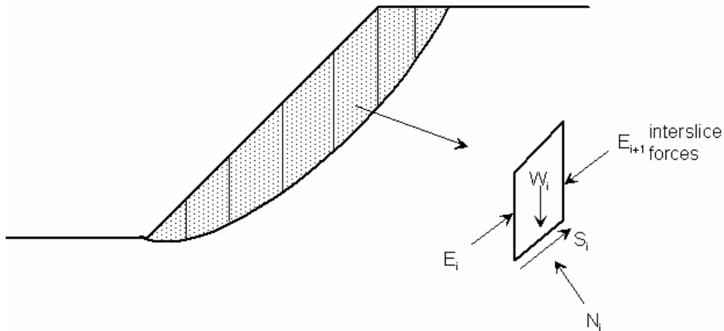
Figure 3.2: Individual slice under equilibrium in an analysis using procedures of slices.
