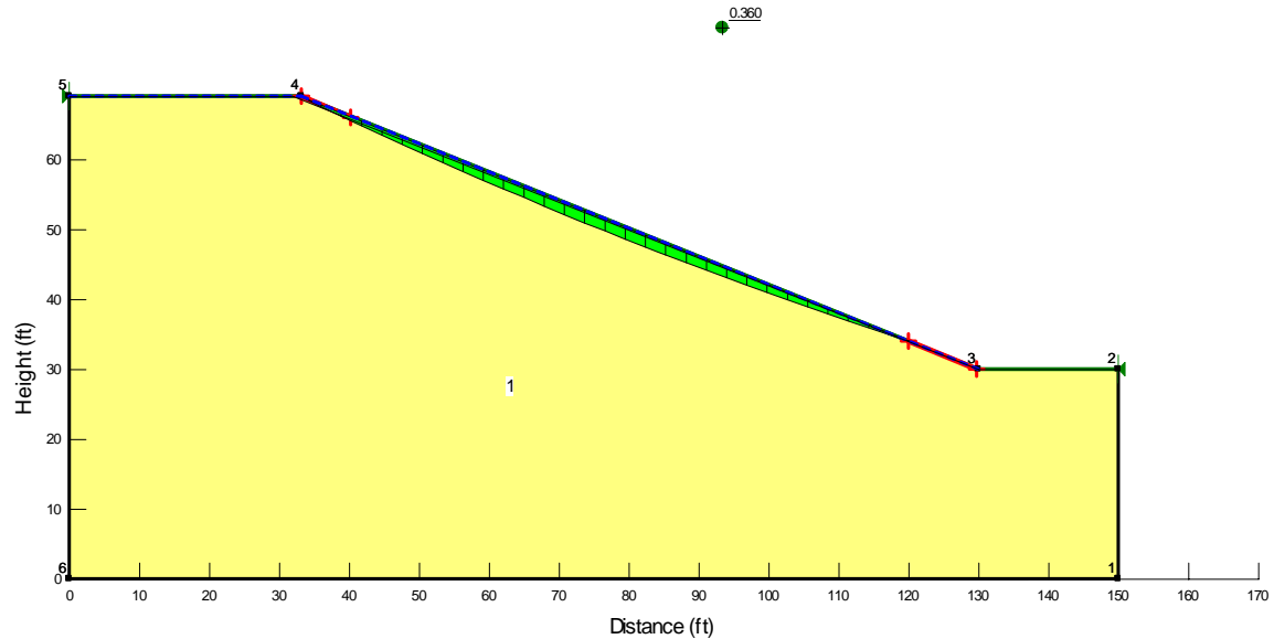
Figure 3.32: Surficial slip surface of the STH-164 slope with saturated homogeneous cohesionless soil ( \phi'=20^\circ ).
