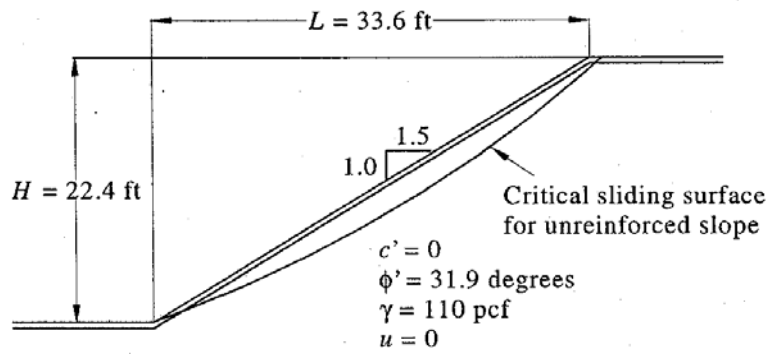
(a) Steep slope
