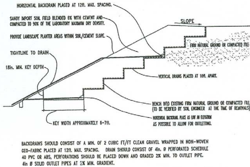
Figure 2.12: Soil cement repair of shallow slope failures (Day, 1997).
