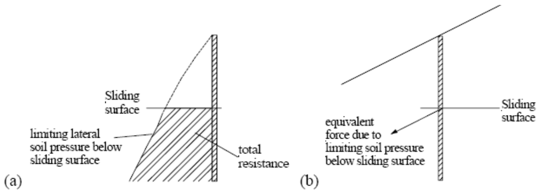
Figure 3.9: Graphical illustration for computing limit anchorage resistance: (a) integral of limiting soil pressure and (b) equivalent total resisting force (after Loehr et al., 2004).
