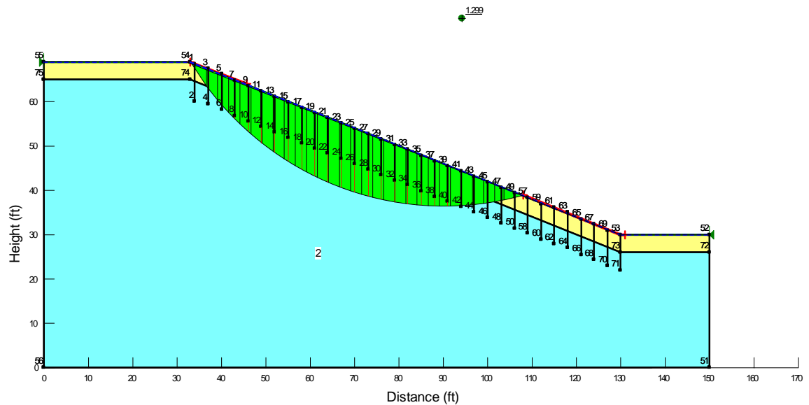
Figure 3.40: Slip surface of STH-164 slope that consists of a dry homogenous soil layer ( c' = 200 psf and \phi' = 15^\circ ) reinforced with 8-ft. vertical structural members.
