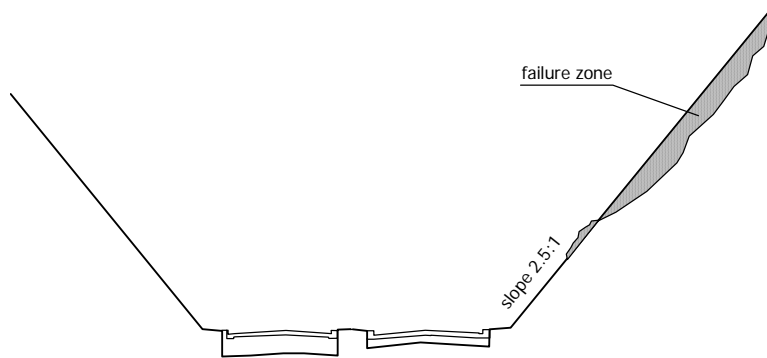
(b) Shallow slope failure at Sta. 299+00
