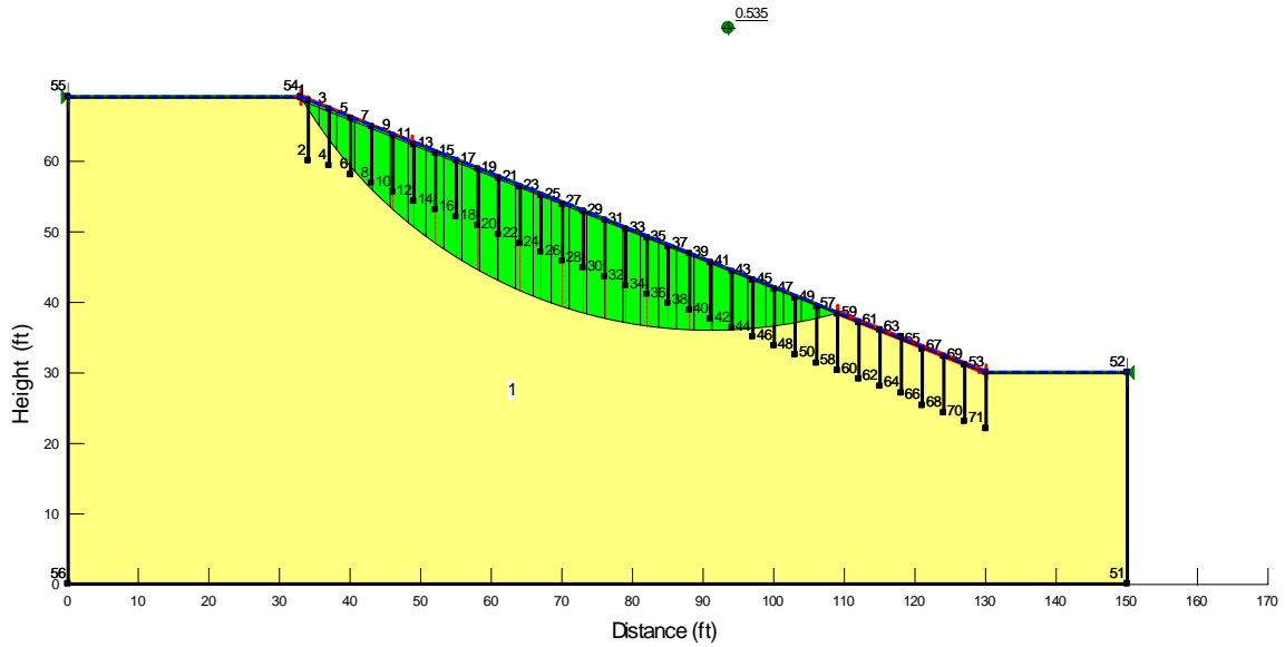
Figure 3.36: Slip surface of STH-164 slope that consists of a saturated homogenous soil layer ( \phi' = 20^\circ ) reinforced with 8-ft. vertical structural members.
