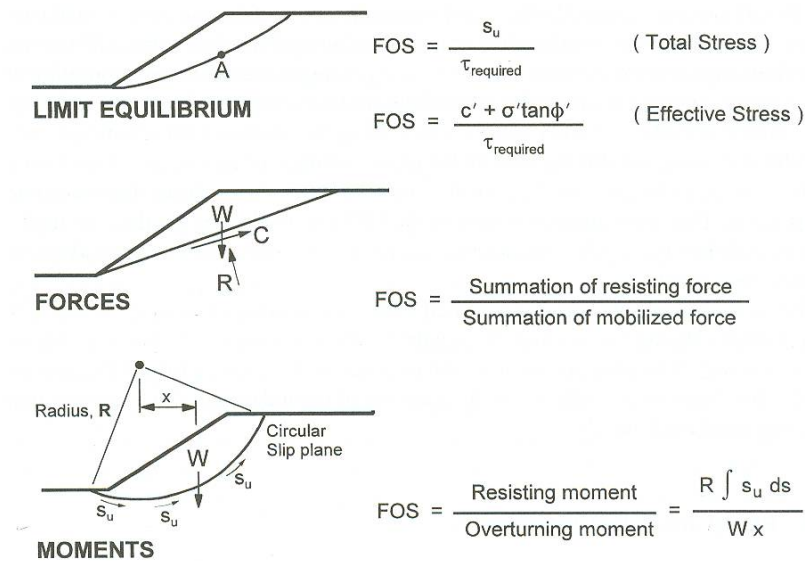
Figure 2.2: Various definitions of factor of safety (Abramson et al., 2002).
