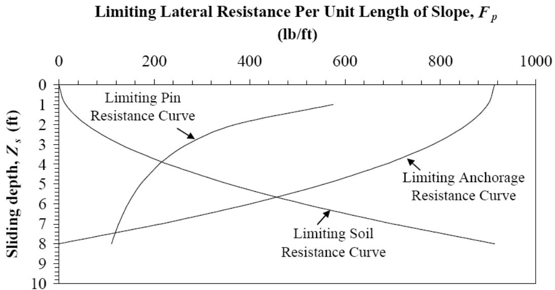
Figure 3.5: Typical distributions of limit resistance developed for the three limit states considered (After Loehr et al., 2004).
