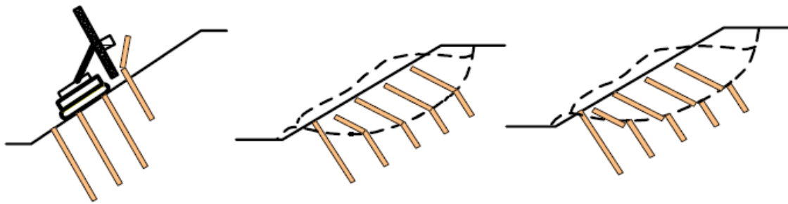
(a) Installation durability (b) Bending and creep failure (c) Shear failure
