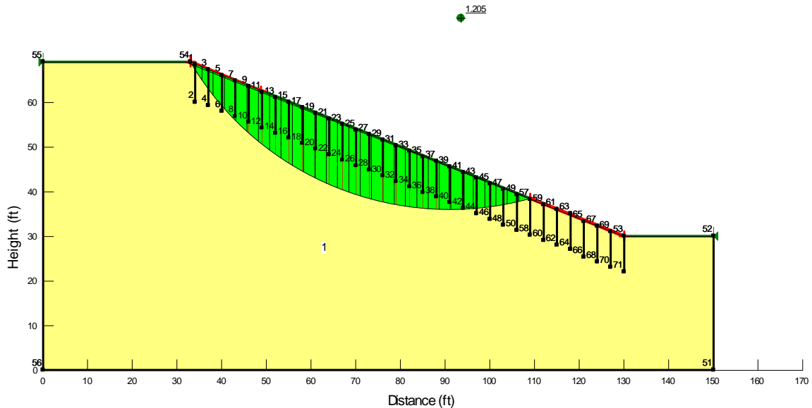
Figure 3.35: Slip surface of STH-164 slope that consists of dry homogenous soil layer ( \phi' = 20^\circ ) reinforced with 8-ft. vertical structural members.
