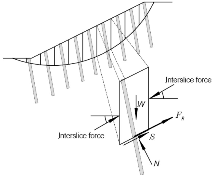
Figure 3.3: Reinforcement force ( F_R ) on an individual slice in the methods of slices (after Loehr and Bowders, 2007).
