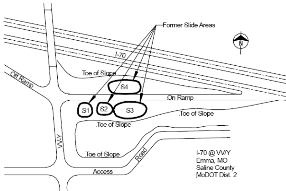
Figure 3.20: Surficial slope failures (S1, S2, S3, and S4) along I-70 embankment near Emma, Missouri (Loehr and Bowders, 2007).
