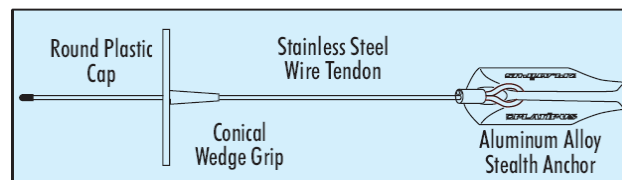
(b) S04E anchor with maximum capacity of 2,200 lbs.
