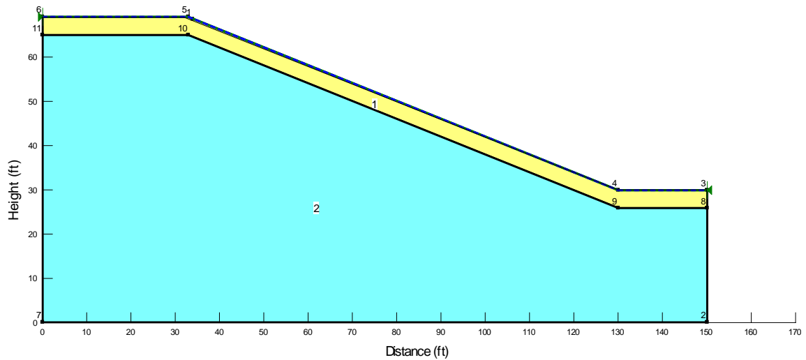
Figure 3.28: Geometry of STH-164 highway slope that consists of an upper soft soil layer over a stiff soil layer with different combinations of shear strength parameters.
