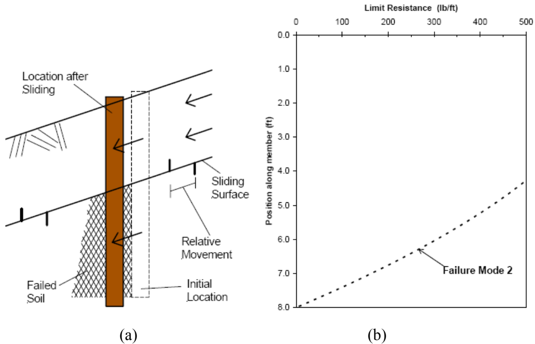
Figure 3.8: (a) Schematic illustrating Failure Mode 2 and (b) Limit resistance curve for Failure Mode 2 (Loehr & Bowders, 2007).
