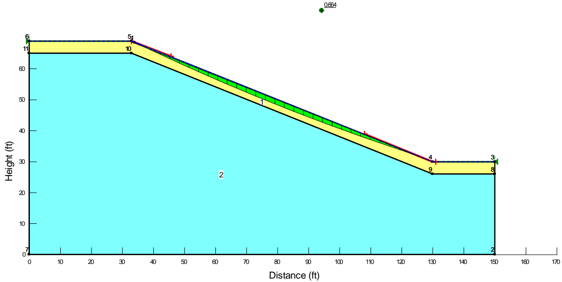
Figure 3.39: Surficial slip surface of the STH-164 slope with upper soft saturated soil ( c' = 20 psf and \phi' = 15^\circ ) and lower stiff saturated soil ( c' = 200 psf and \phi' = 28^\circ ).
