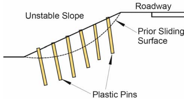
Figure 2.14: Profile of recycled plastic pins stabilizing a potential sliding surface (Loehr et al., 2000).
