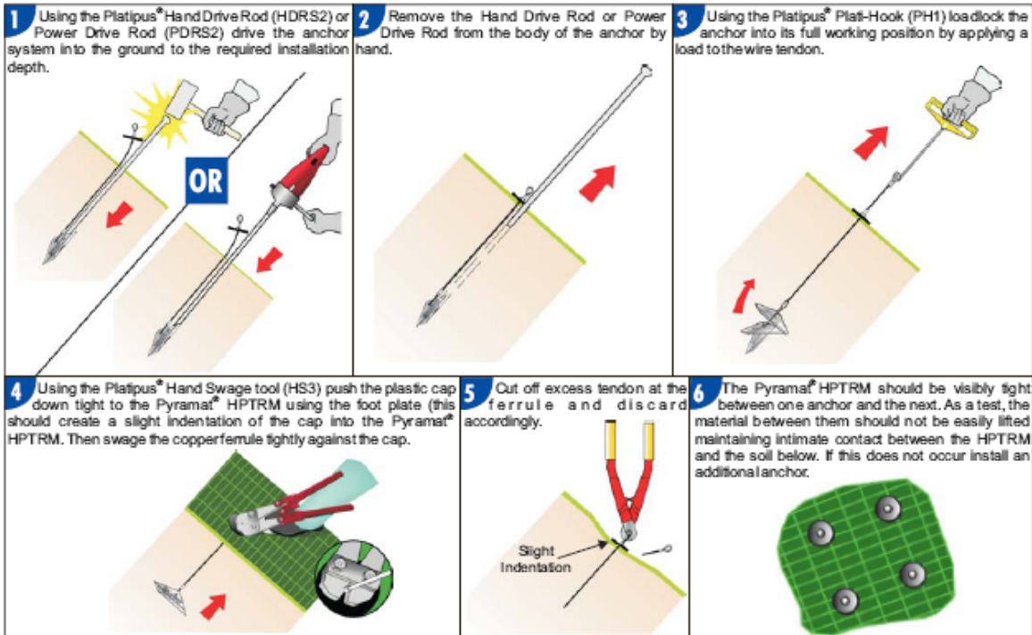
Figure 2.23: Installation of earth anchor (Platipus, 2007).
