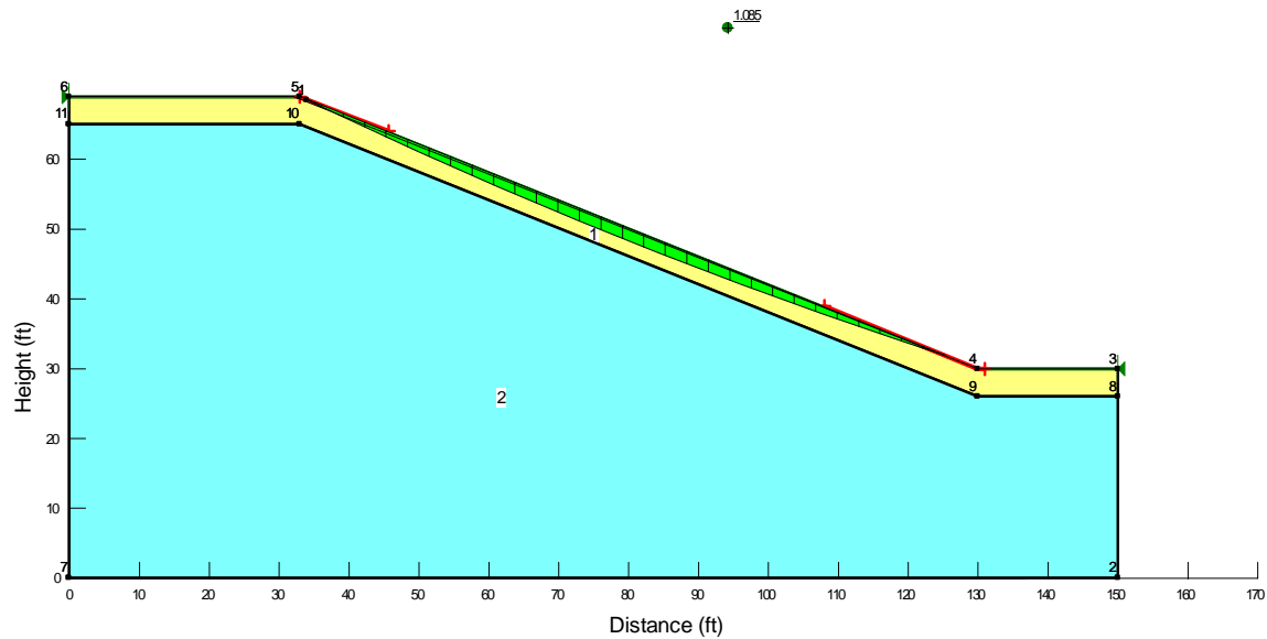
Figure 3.38: Surficial slip surface of the STH-164 slope with upper soft dry soil ( c' = 20 psf and \phi' = 15^\circ ) and lower stiff dry soil ( c' = 200 psf and \phi' = 28^\circ ).
