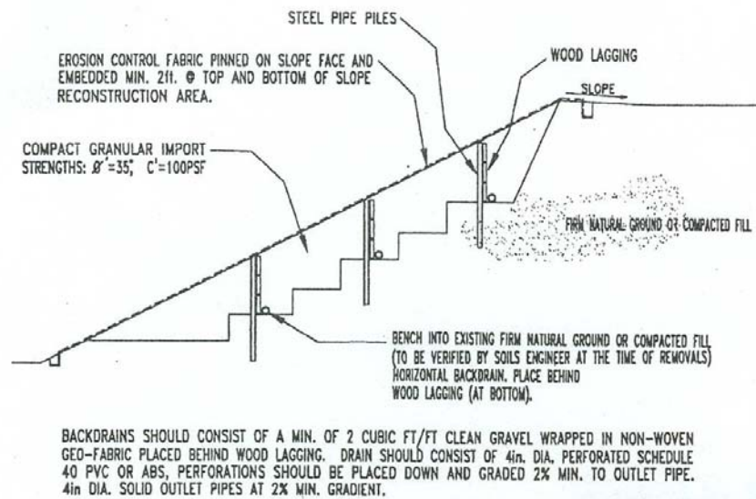
Figure 2.10: Pipe pile and wood lagging repair (Day, 1997).
