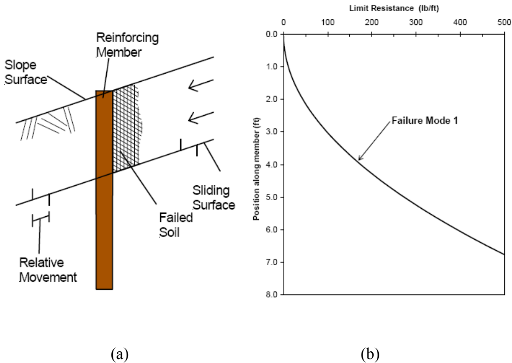
Figure 3.6: (a) Schematic illustrating Failure Mode 1 and (b) Limit resistance curve for failure mode 1 (Loehr & Bowders, 2007).
