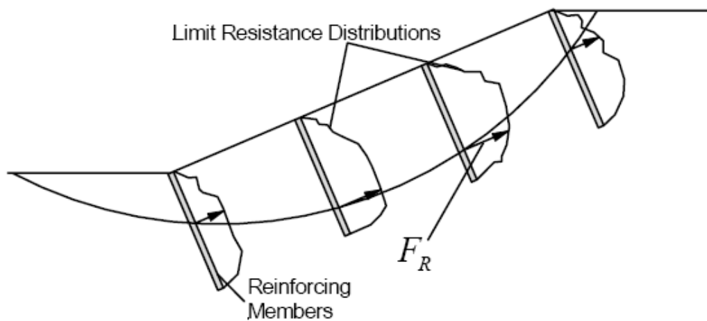
Figure 3.4: Example of distributions of limit resistance for multiple members in a reinforced slope (after Loehr and Bowders, 2007).
