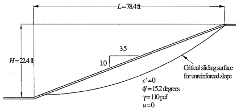
(c) Flat slope
