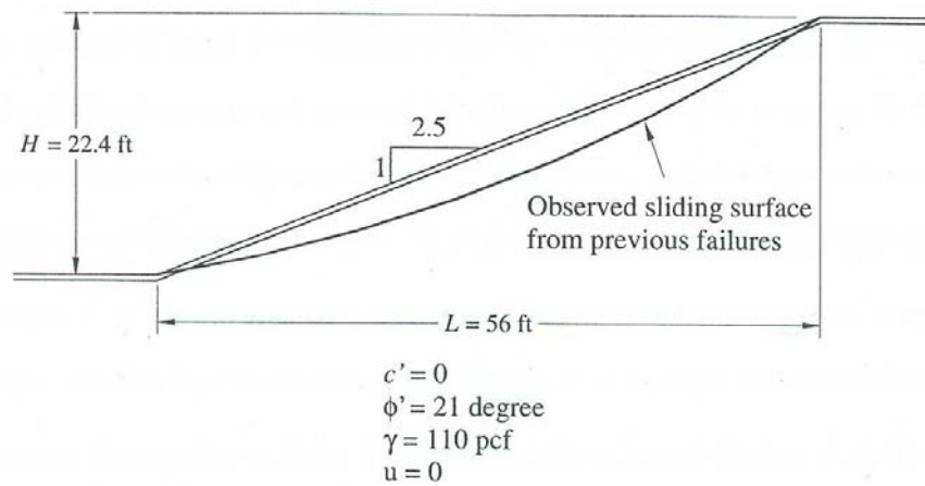
Figure 3.13: Estimated slope geometry and conditions and the observed sliding surface used in the analysis (after Liew, 2000).
