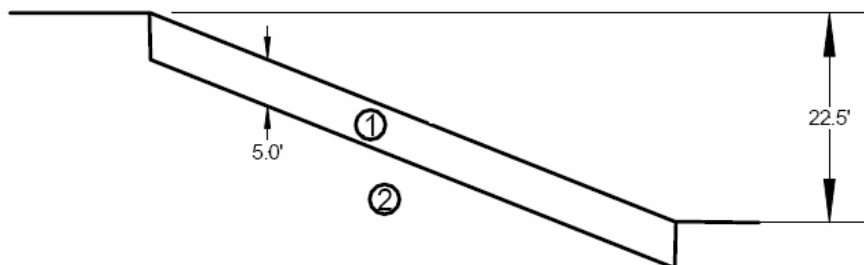
Figure 3.23: Slope section assumed in stability condition B (after Loehr and Bowders, 2007).
