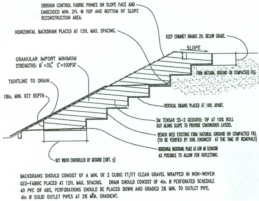
Figure 2.11: Repair of surficial slope failure by geogrid (Day, 1997).
