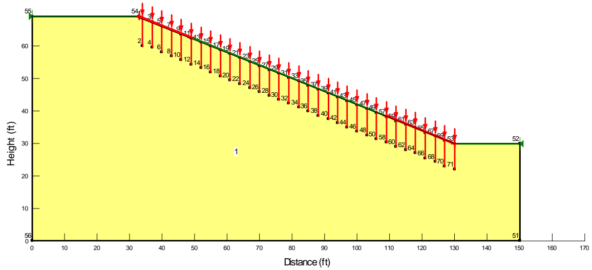
Figure 3.29: Geometry of STH-164 highway slope that consists of one soft homogeneous soil layer stabilized with vertical structural members.
