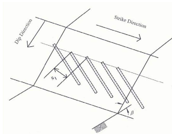
Figure 3.11: Slope reinforced with a single row of reinforcing members spaced equally in the longitudinal (strike) direction (after Liew, 2000).
