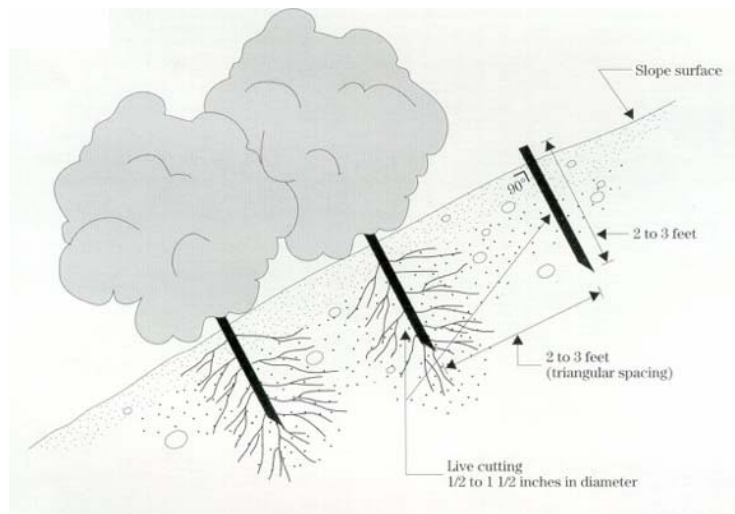
(a) Live staking details
