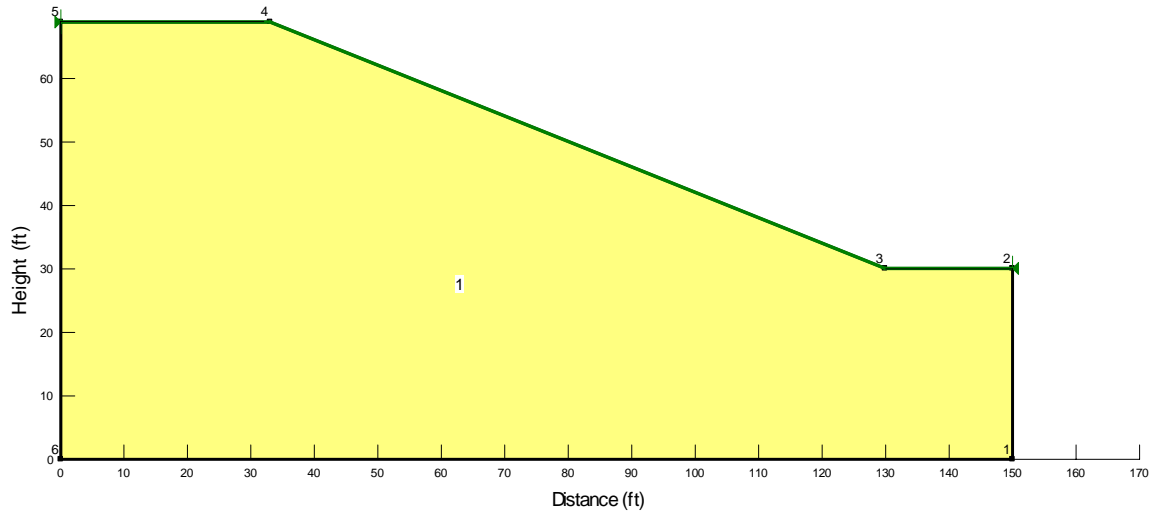
Figure 3.27: Geometry of STH-164 highway slope that consists of one soft homogeneous soil layer with different combinations of shear strength parameters.
