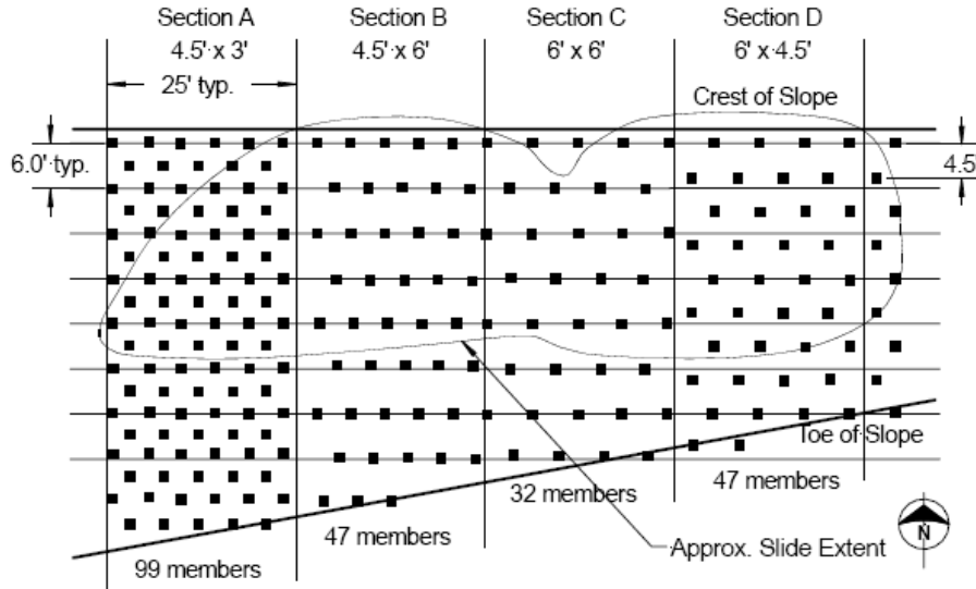
Figure 3.22: Plan view of selected stabilization schemes for slide area S3 at the I-70 Emma test site (Loehr and Bowders, 2007).
