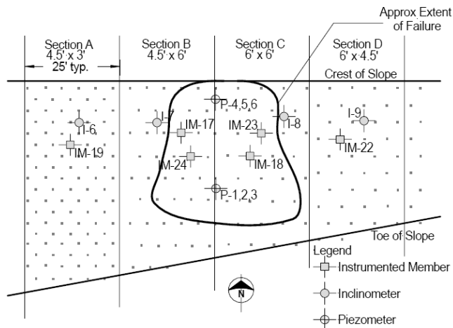
Figure 3.26: Approximate extent of failure at I-70 Emma site (Loehr and Bowders, 2007).
