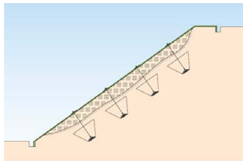
(c) Installing mechanical earth anchors through the mat below the slip surface
