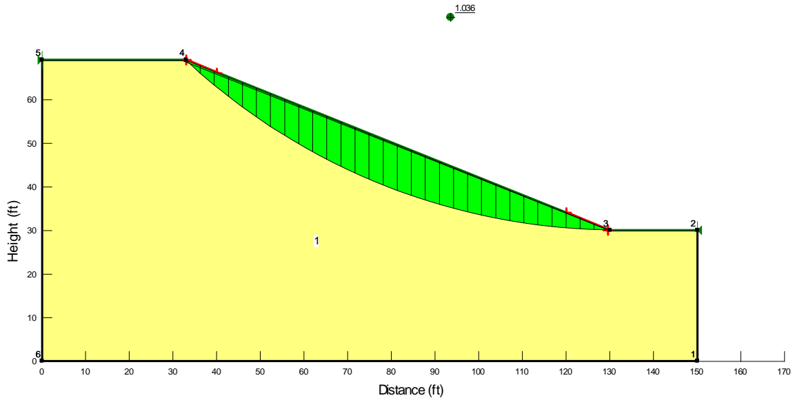
Figure 3.33: Relatively deep slip surface of the STH-164 slope when analysis is conducted with dry soft homogeneous soil layer ( c' = 20 psf and \phi' = 20^\circ ).
