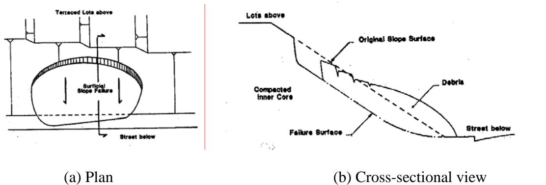
Figure 2.5: Illustration of typical surficial slope failure (Day, 1997).
