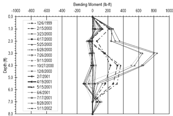
Figure 3.25: Measured bending moments in instrumented member IM-H at I-70 Emma test site during Phase I (Loehr and Bowders, 2007).
