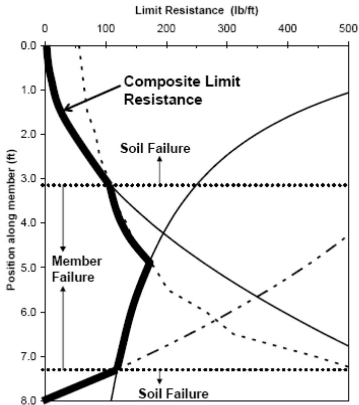
Figure 3.10: Composite limit lateral resistance distribution for recycled plastic reinforcing member (After Loehr & Bowders, 2007).
