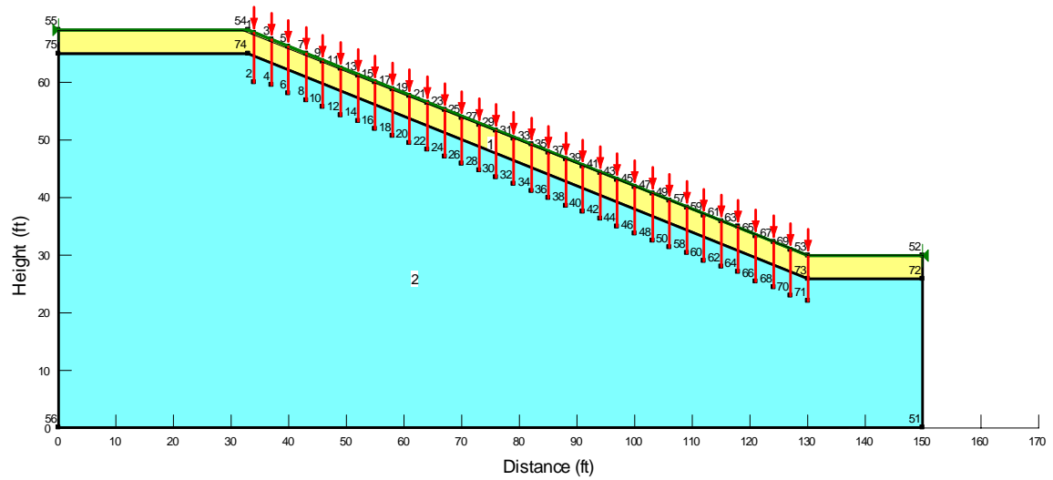
Figure 3.30: Geometry of STH-164 highway slope that consists of an upper soft soil layer over a stiff soil layer stabilized with vertical structural members.
