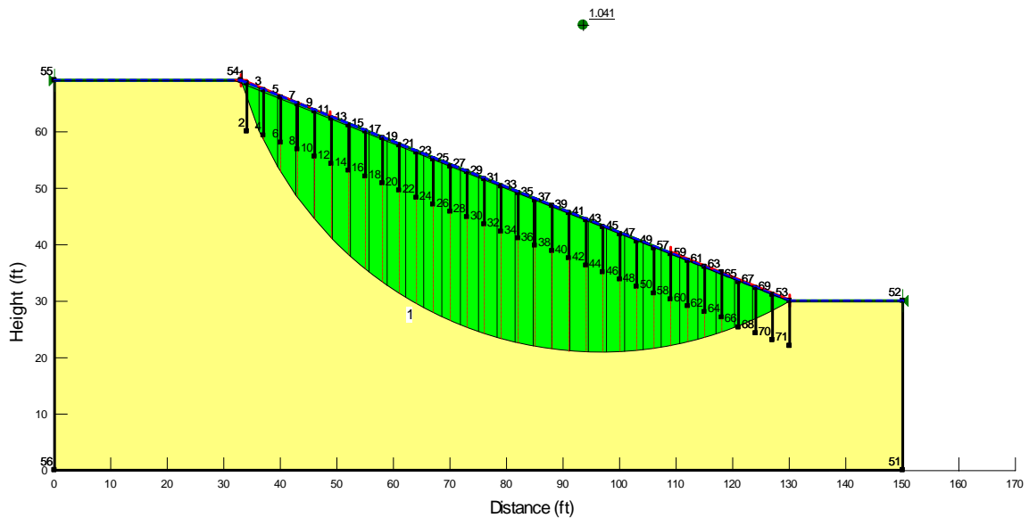
Figure 3.37: Slip surface of STH-164 slope that consists of a saturated homogenous soil layer ( c' = 200 psf and \phi' = 20^\circ ) reinforced with 8-ft. vertical structural members.
